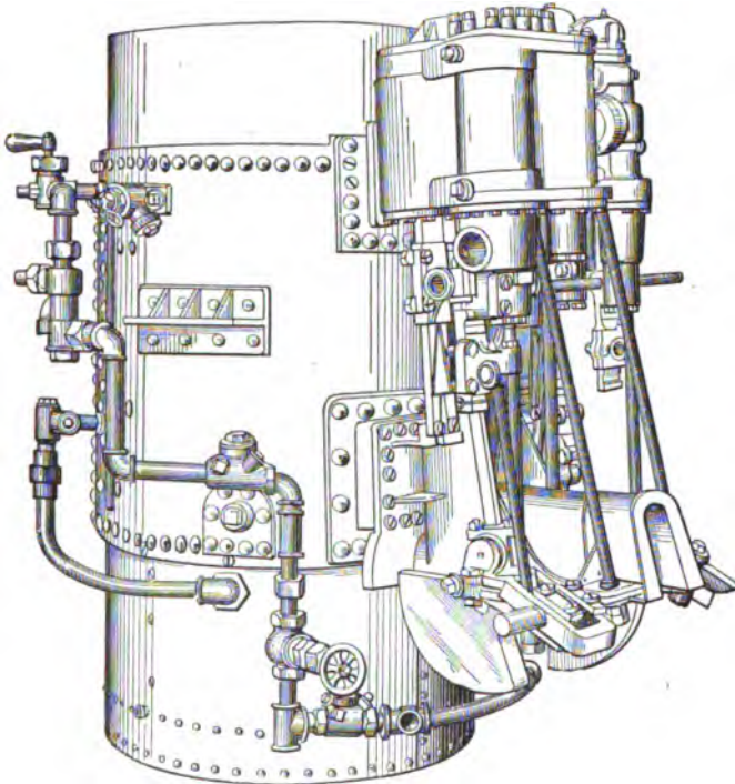
FIG. 271. —Boiler and Burner of the McKay Carriage showing Compound Engine attached. The feed water for this boiler passes through a waterleg around and above the burner, being fed at nearly 200° temperature. The engine may be run either compound or simple, but the two cylinders are connected by a superheater tube passing over the upper tube plate of the boiler, somewhat as in Fig. 149. The advantages of hanging the engine direct to the boiler are the avoidance of flexible connections and in permitting the cylinders to be steam-jacketed direct with live steam.
